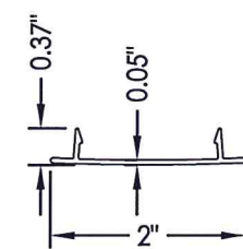
5 MULLION COVER
