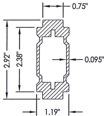
1 MULLION (5901) 6063-T5 ALUM
