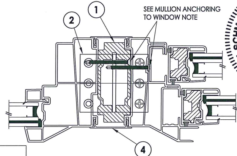
3 2 HORIZONTAL CROSS SECTION @ MULLION ANCHOR BRACKET (SHOWN w/ FIXED FRAME & DOUBLE HUNG)
