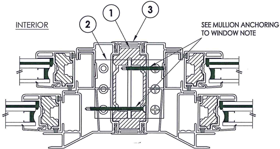
1 2 HORIZONTAL CROSS SECTION @ MULLION ANCHOR BRACKET (SHOWN w/ DOUBLE HUNG FRAME)
