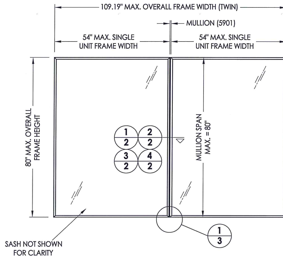
MULLED TWIN WINDOW UNITS SHOWN (Multiples also approved)
