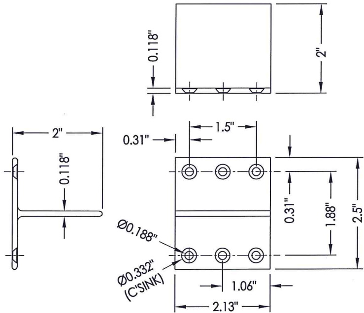
2 MULLION ANCHOR BRACKET (5950) 6063-T5 ALUM
