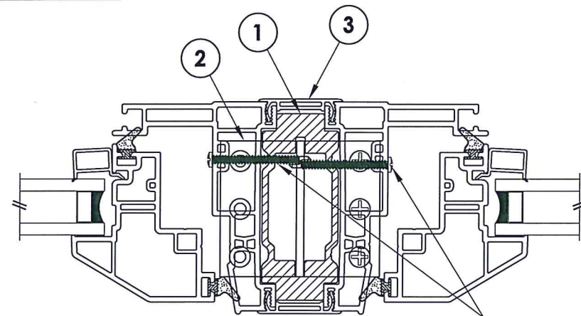
4 2 HORIZONTAL CROSS SECTION @ MULLION ANCHOR BRACKET (SHOWN w/ CASEMENT/AWNING FRAME)
