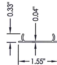
4 MULLION COVER
