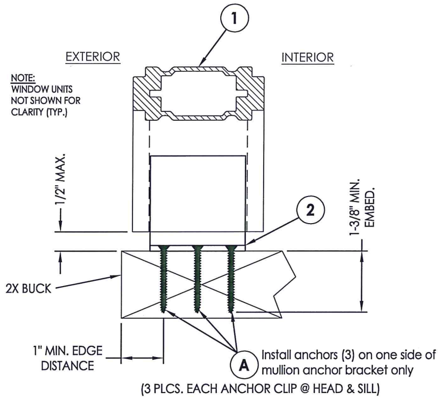
1 HORIZONTAL CROSS SECTION 3 MULLION ANCHOR BRACKET DETAIL 2X BUCK ANCHORING
